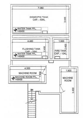
MACHINE ROOM / WATER TANK PLAN
