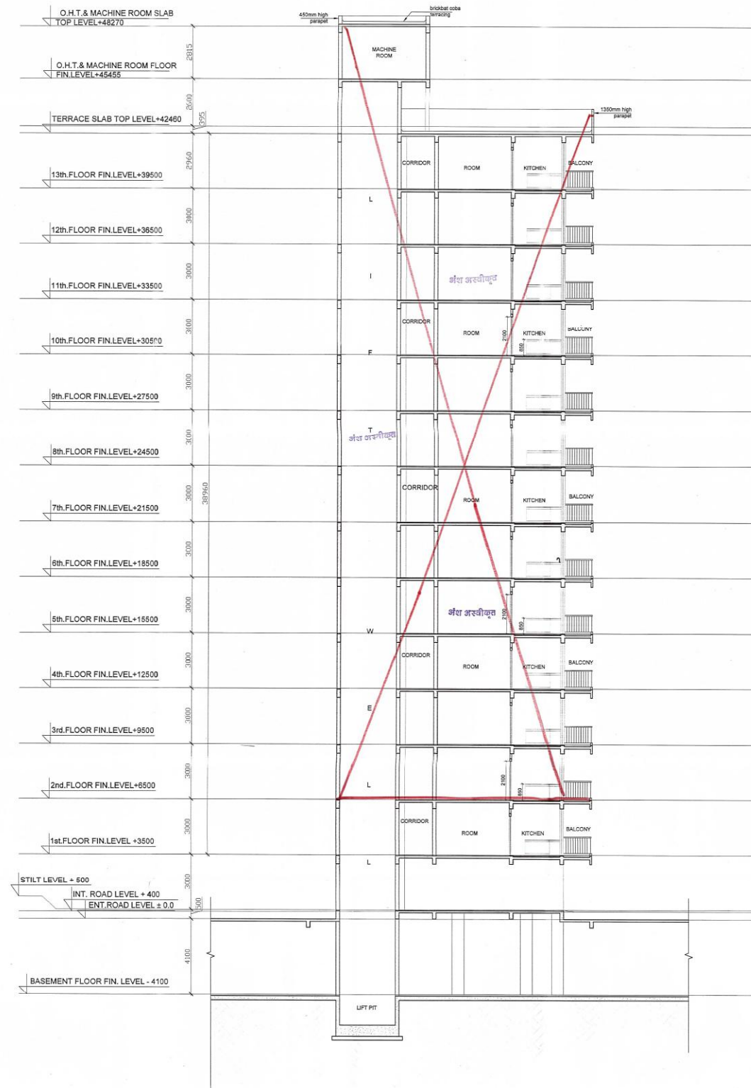
SECTION B-B
